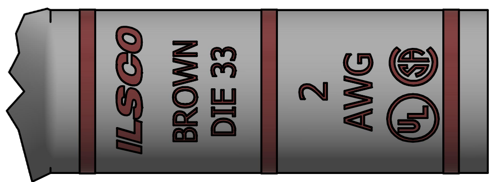
DETAIL E TOP & BOTTOM INK MARK
